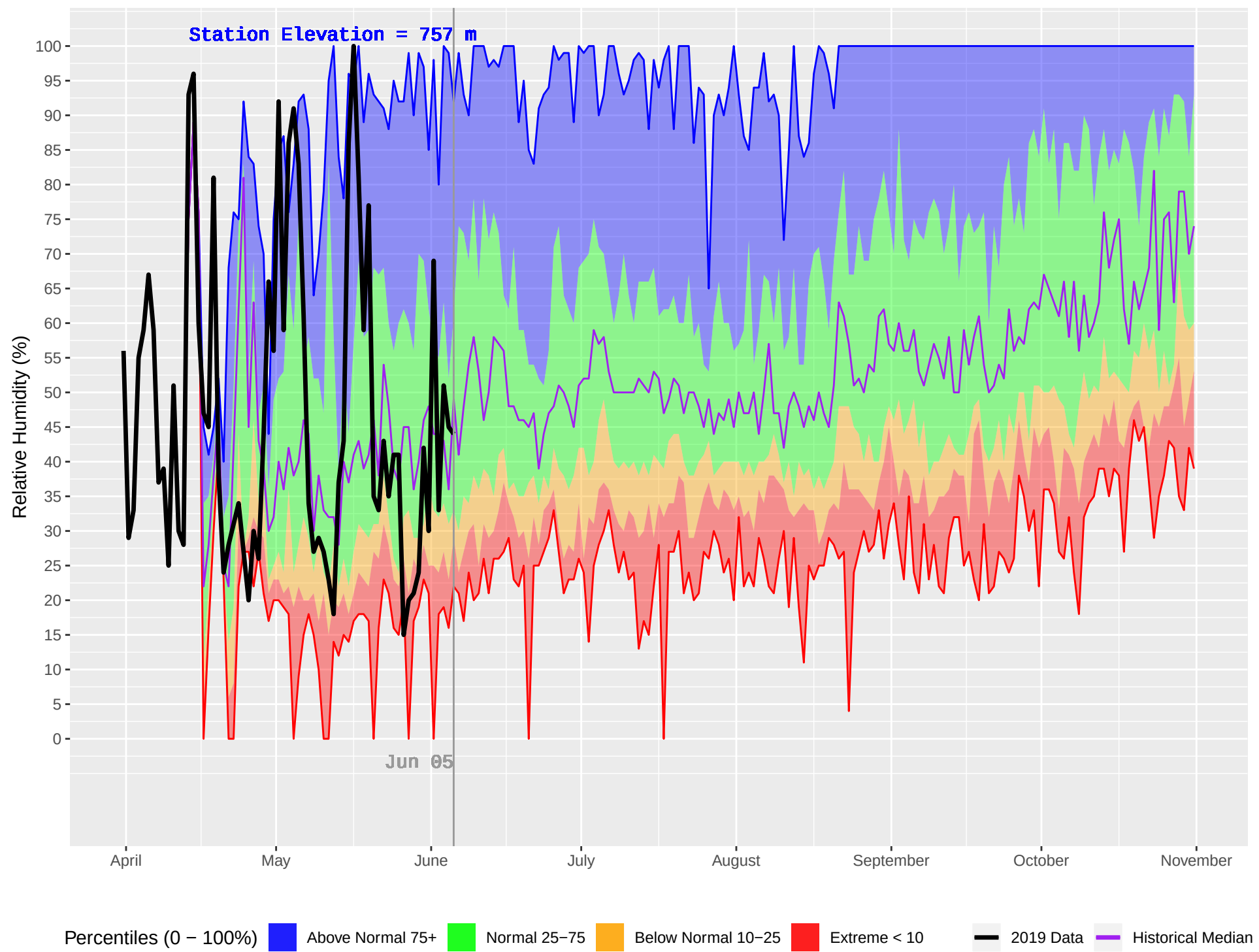
LEMORAY (140) : Historical (1988–2018) and Current (2019) Daily Relative Humidity
