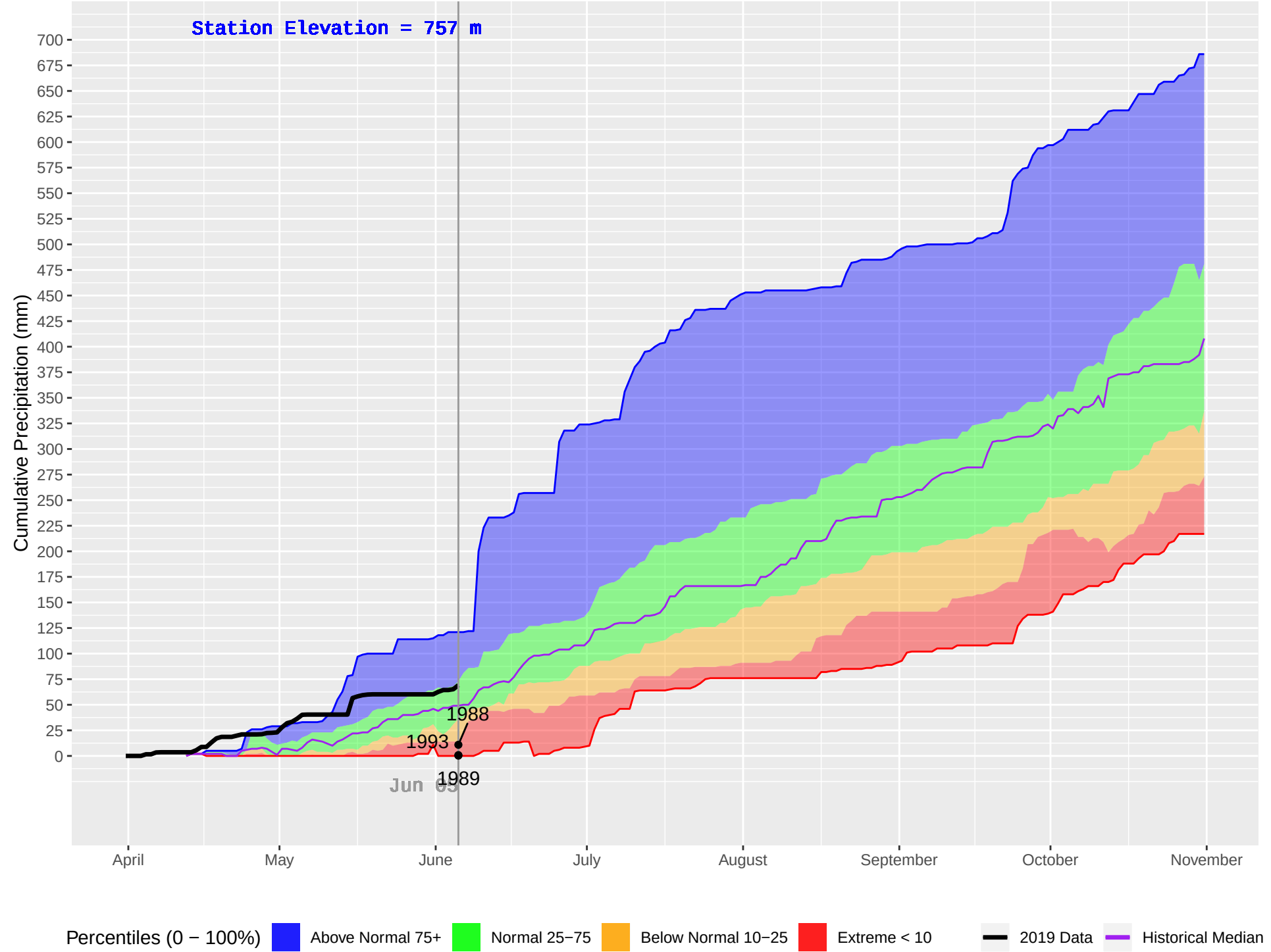
LEMORAY (140) : Historical (1988–2018), Current (2019) Daily Cumulative Precipitation
