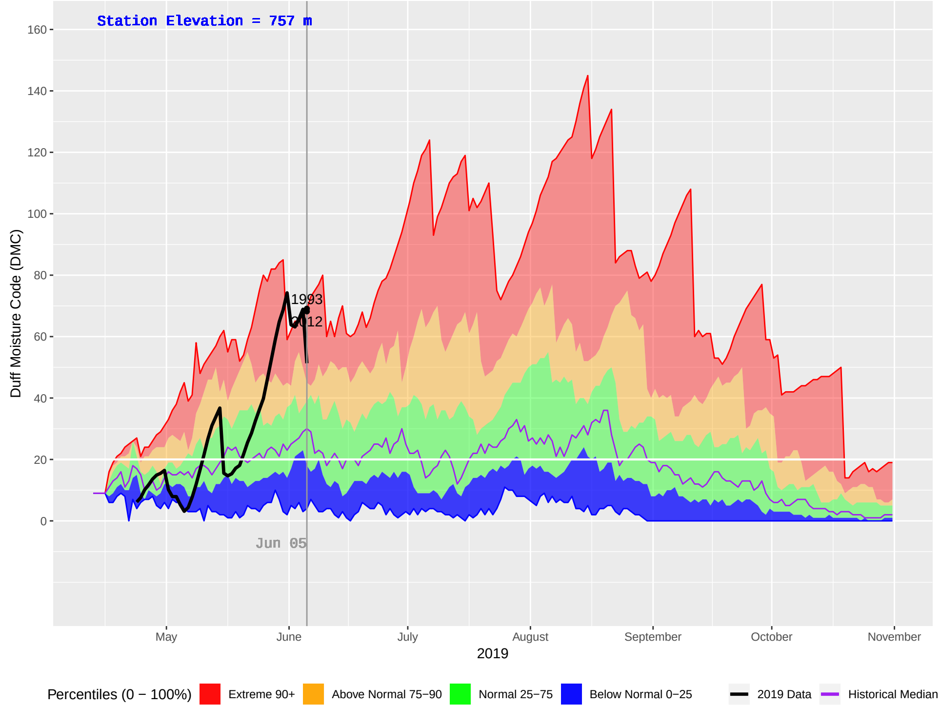
LEMORAY (140) : Historical (1988–2018), Current (2019) Daily Duff Moisture Code (DMC)
