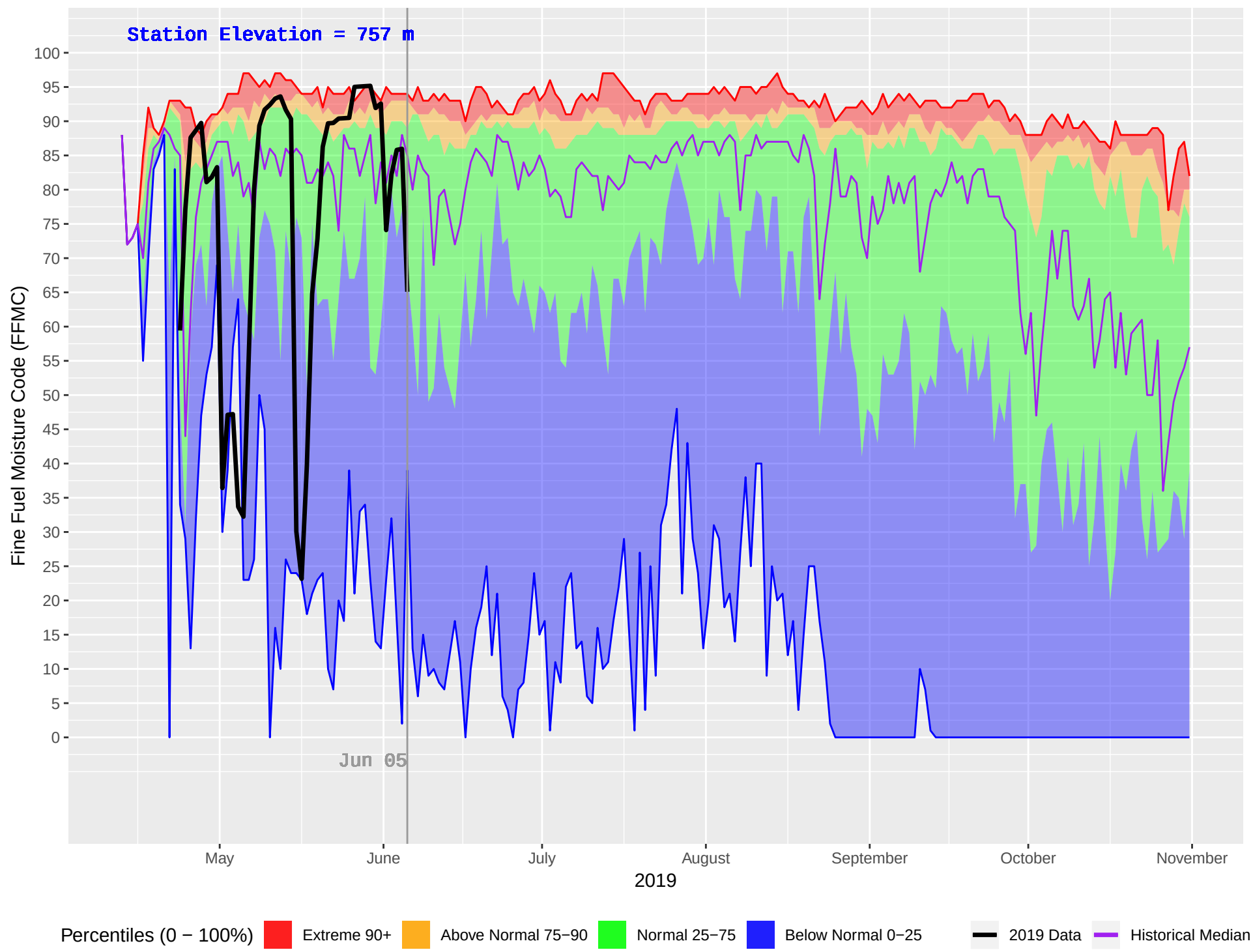
LEMORAY (140) : Historical (1988–2018) and Current (2019) Daily Fine Fuel Moisture Code (FFMC)
