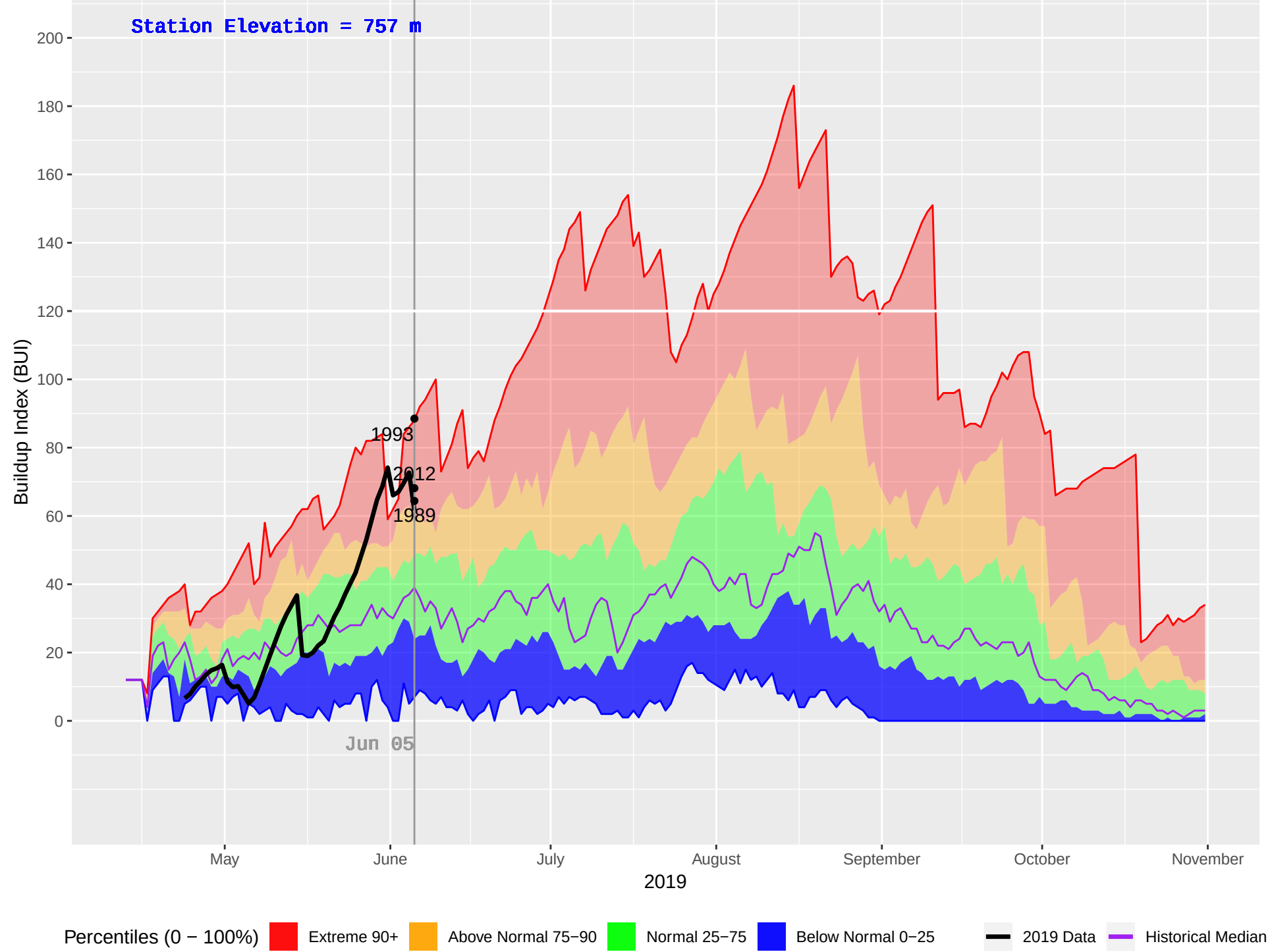
LEMORAY (140) : Historical (1988–2018), Current (2019) Daily Buildup Index (BUI)
