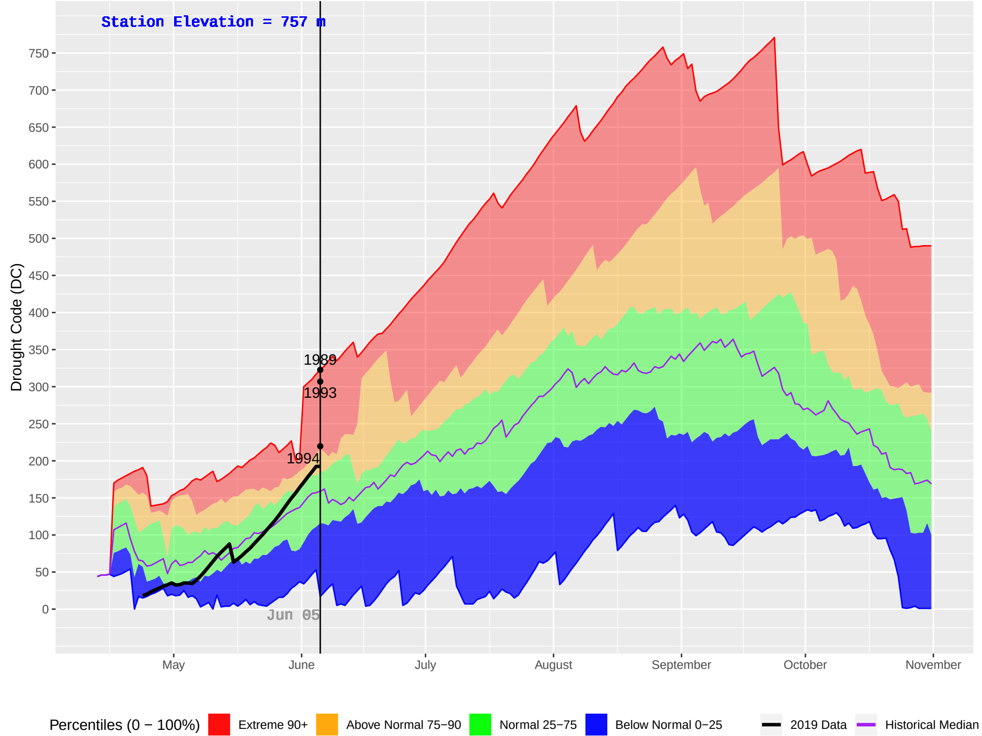
LEMORAY (140) : Historical (1988–2018) and Current (2019) Daily Drought Code (DC)
